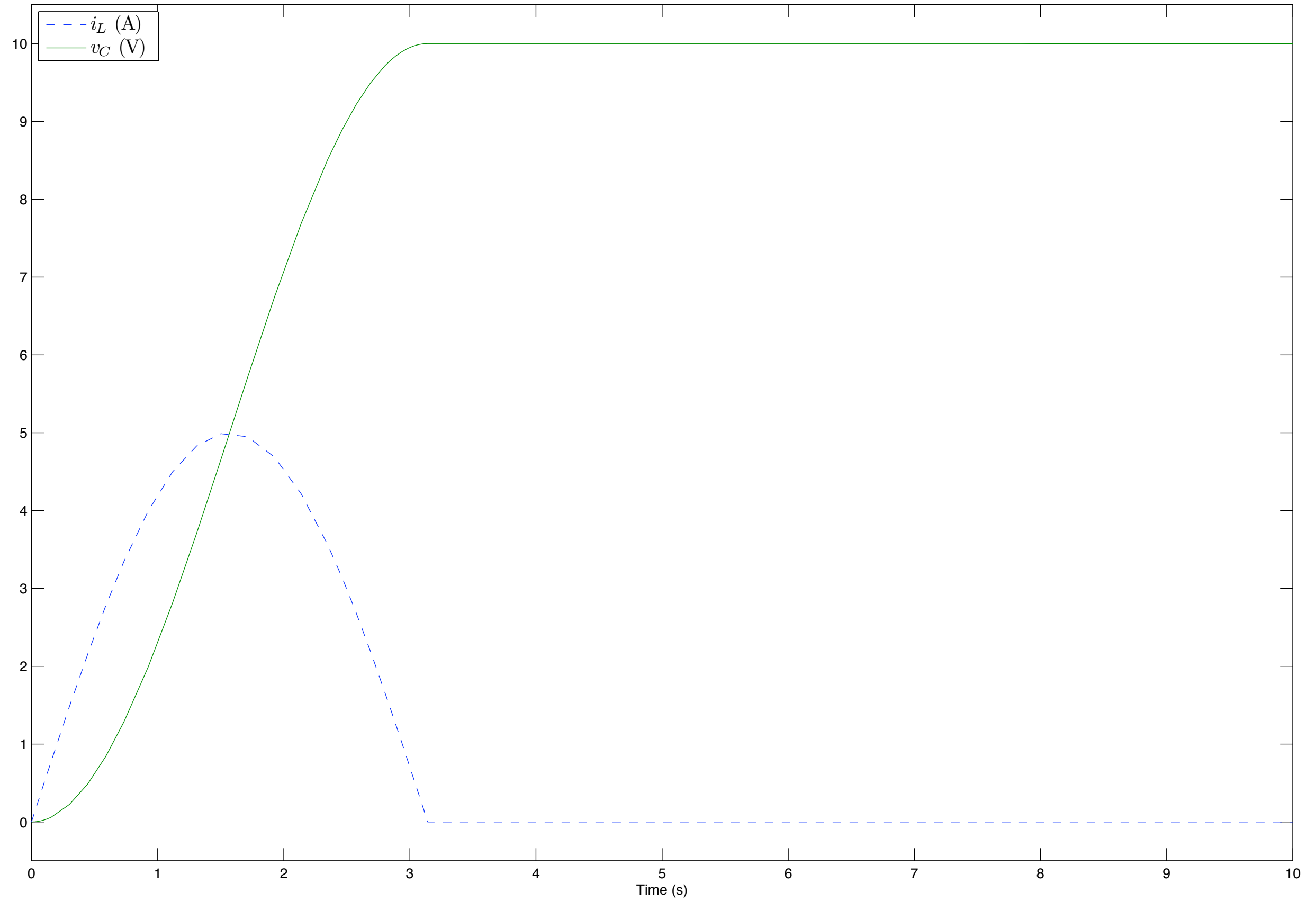
LC + diode summary ( L = 1 H, C = 1 F, v_{in} = 5 V)
