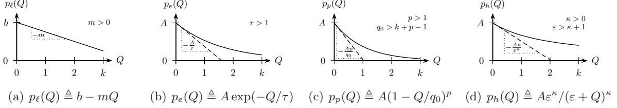
Figure 2.3: Sample stabilizing payment (i.e., inverse demand) functions.
