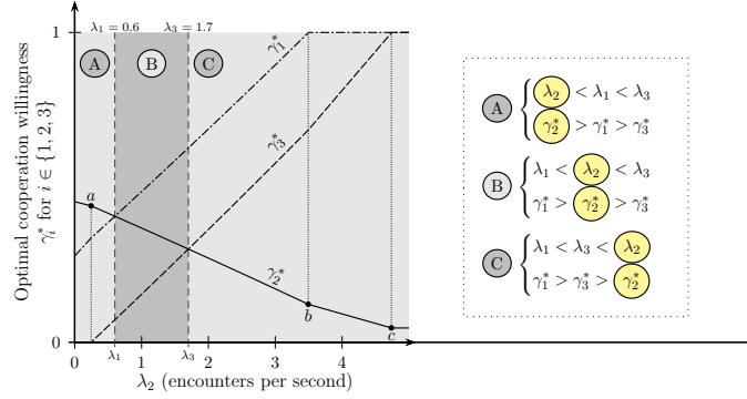
Figure 2.5: AAV optimal cooperation willingness as encounter rates vary.
